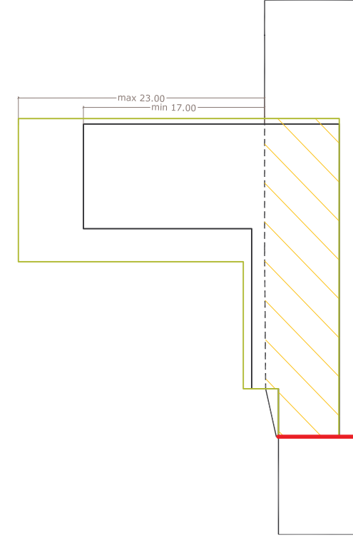
Section CC'
